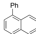
1-phenylnaphthalene
